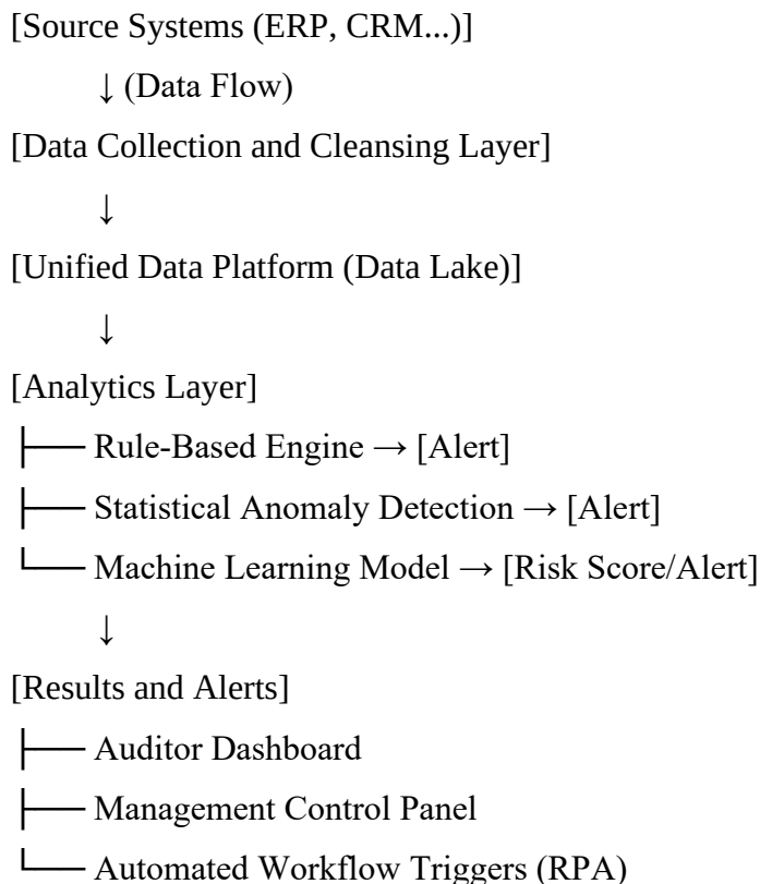
Figure 2: Architectural Flow of an AI-Powered Continuous Auditing System
